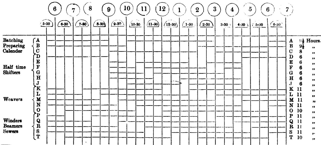
Diagram shewing General Arrangement for Multiple Shift Working.
